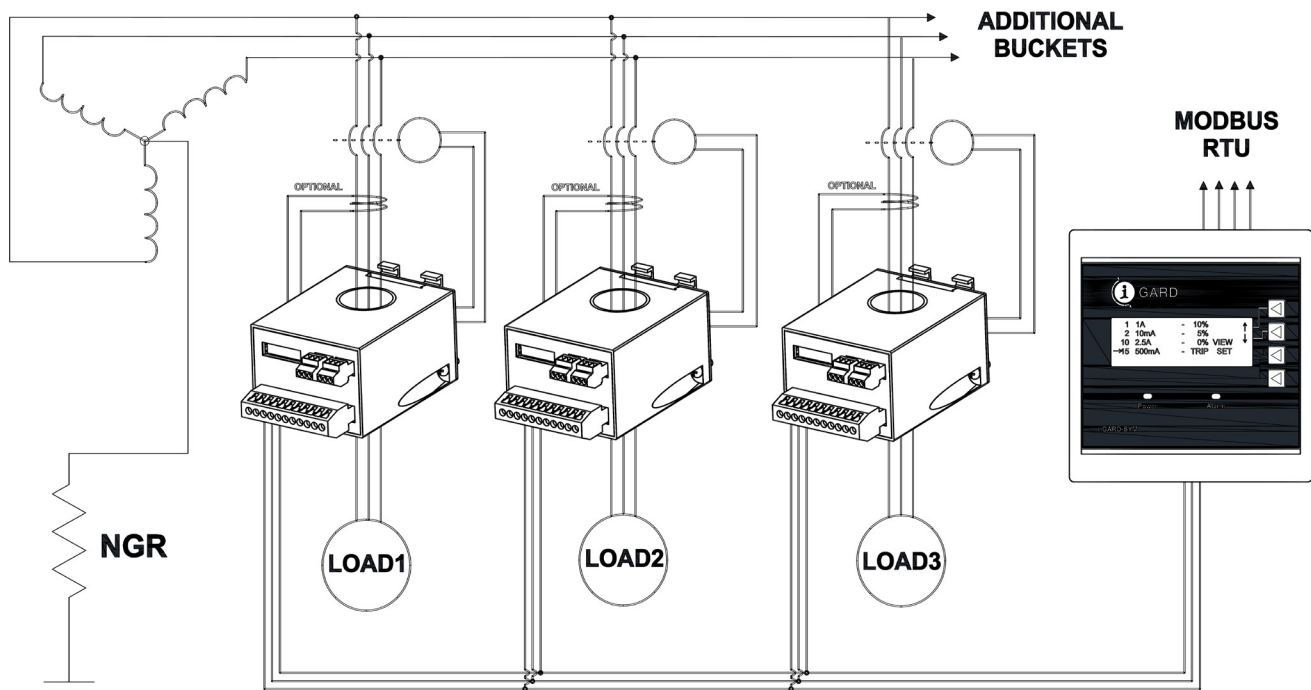
Figure 4.3 mGARD-10-X2 relay monitoring a resistance grounded system. Operating in Failsafe mode, manual reset
