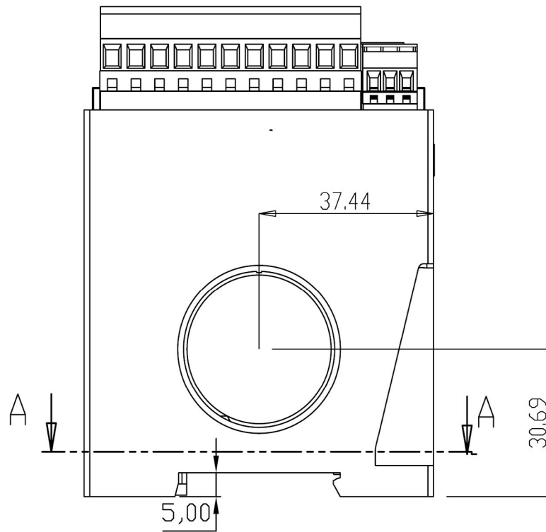
Figure 8.5: mGARD-10-C, mGARD-10-C1 Side Dimensions (Inches)
