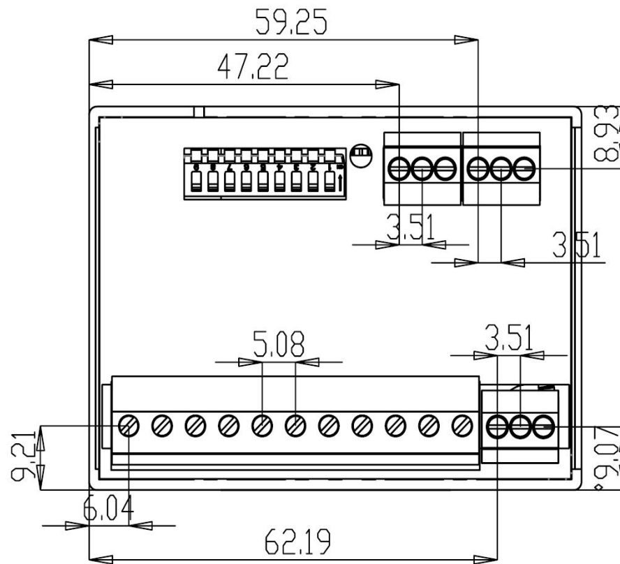
Figure 8.3: mGARD-10-C, mGARD-10-C1 Top Dimensions (Inches)
