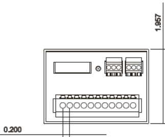
Figure 8.0: mGARD-10-A, mGARD-10-A1 Dimensions (Inches)
