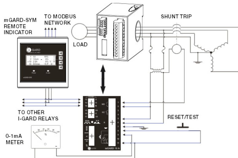
Figure 4.0: mGARD-10-X wired for internal current transformer, non-failsafe operating mode.
