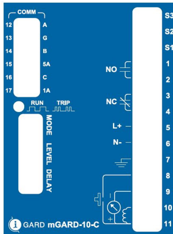
Figure 8.6: mGARD-10-C, mGARD-10-C1 Faceplate
