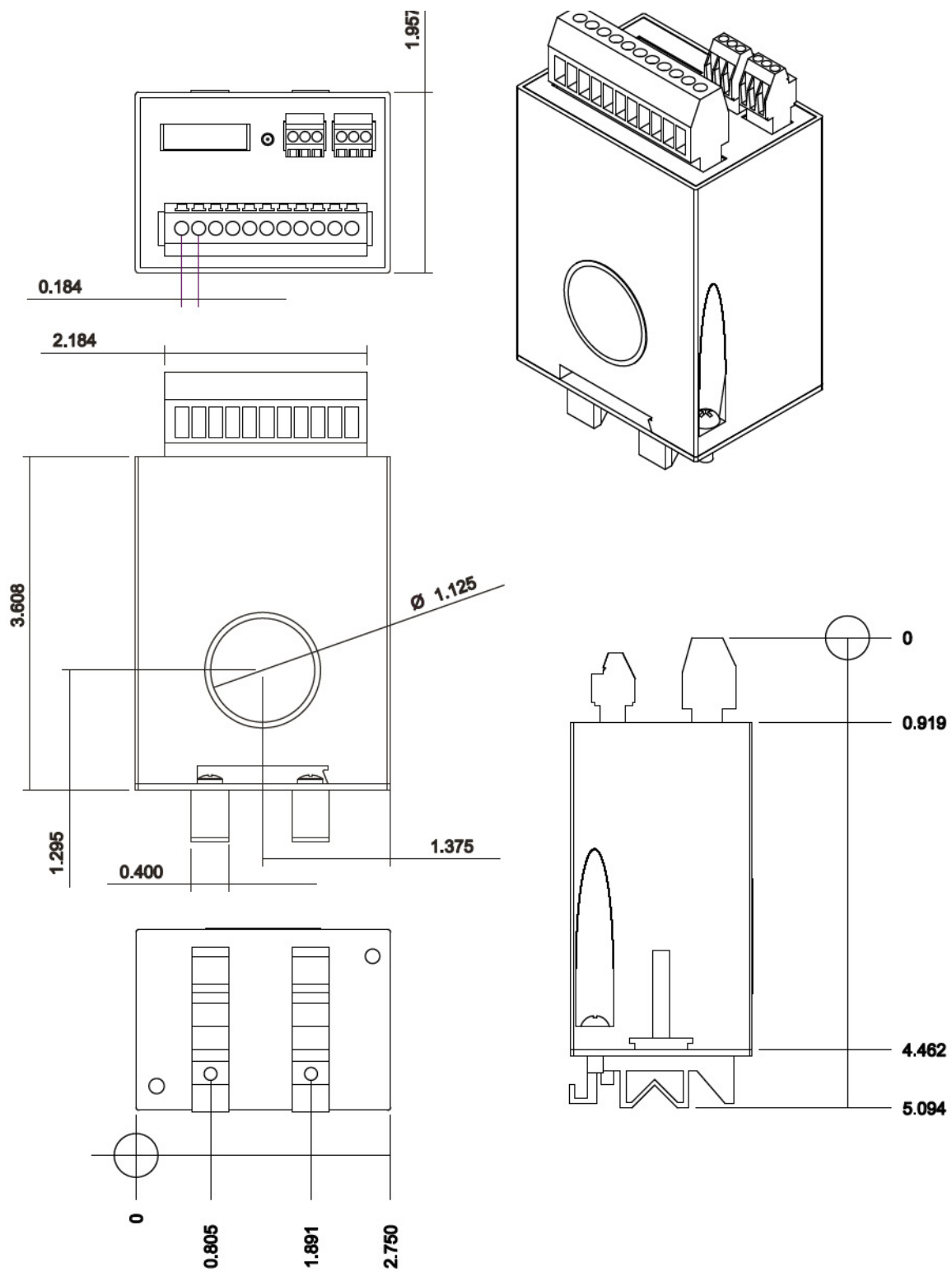
Figure 8.2: mGARD-10-A2 Dimensions (Inches)
