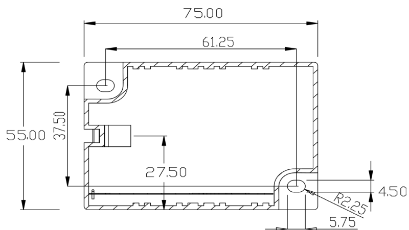
Figure 8.4: mGARD-10-C, mGARD-10-C1 and mGARD-10-C2 Bottom Dimensions (Inches)
