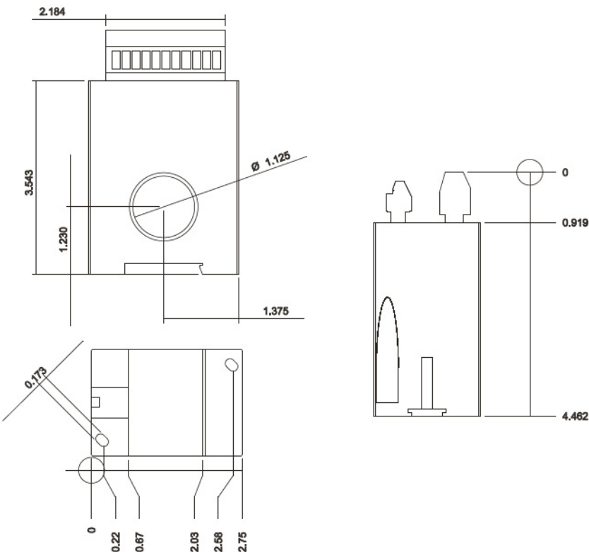
Figure 8.1: mGARD-10-A, mGARD-10-A1 Dimensions (Inches)
