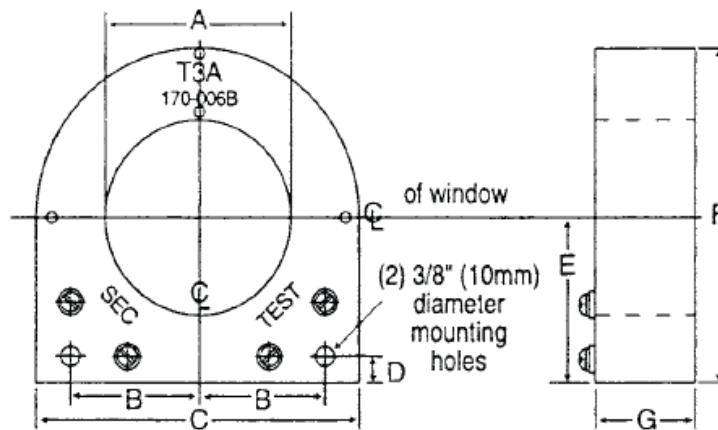
Figure 4: Type T3A, T6A, T9A
