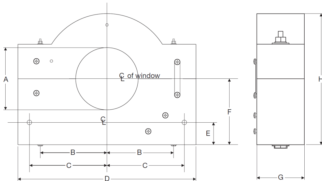
Figure 5: Type T3A-S, T6A-S
