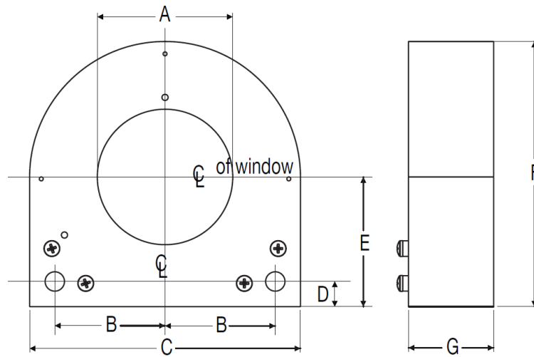
Figure 2: Type T3B, T5B
