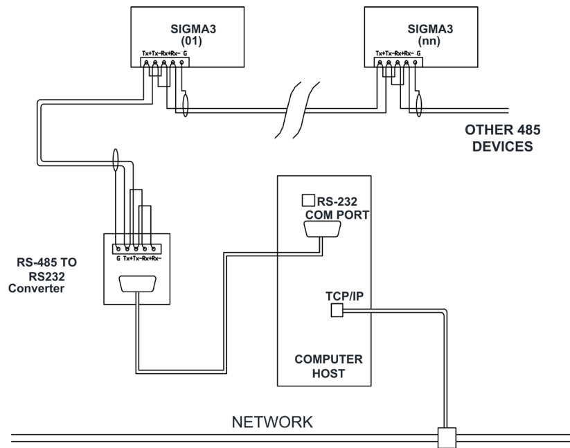
Figure 8.1 (b): Alternate 2-wire MODBUS Communication Connection
