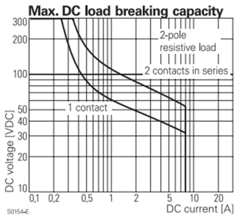
Figure 11.1: Maximum switching power Volts and Amps (AC/DC)
