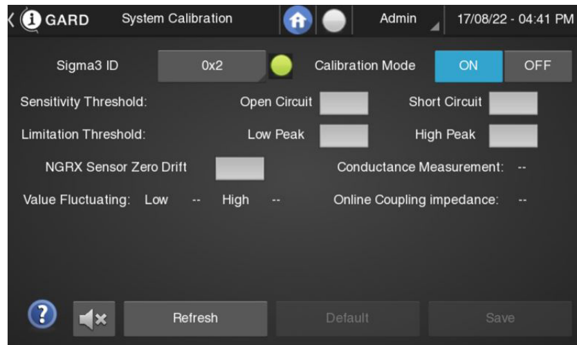
Figure 10.11: SIGMA 3 System Calibration Screen
