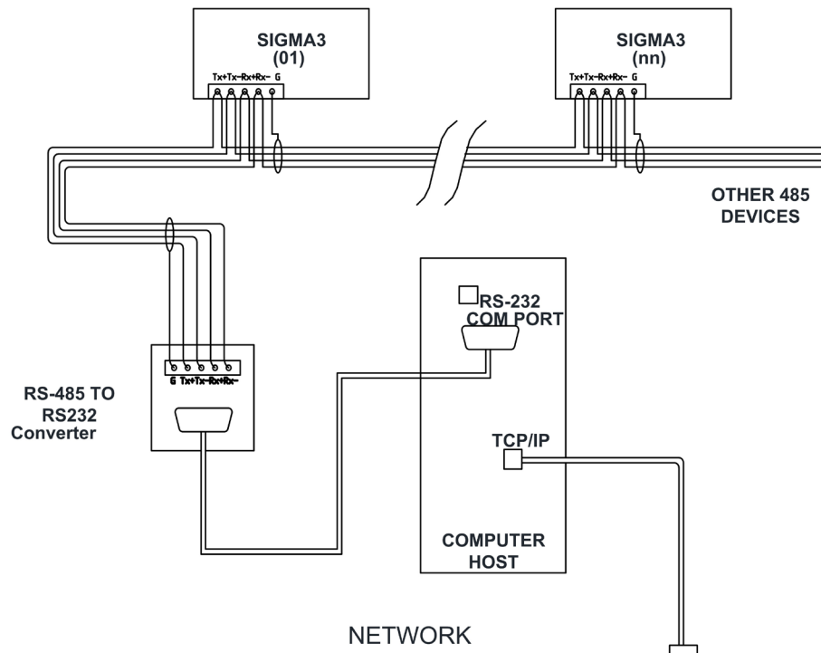
Figure 8.1 (a): Preferred 4-wire MODBUS Communication Connection
