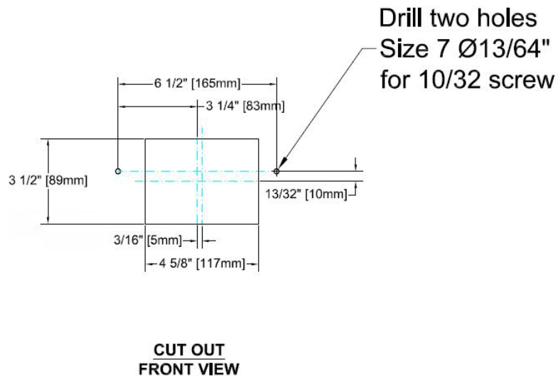
Figure 12.3: SIGMA 3-TDM Mounting Details
