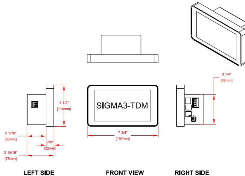
Figure 12.2: SIGMA 3-TDM Dimensional Drawings
