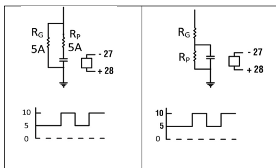
Figure 3.3: The creation of a pulse signature by cycling the let-through current under various arrangements
