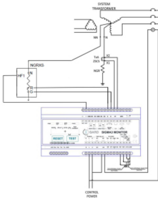
Figure 3.1: SIGMA 3 Typical System Diagram (HRG System)
