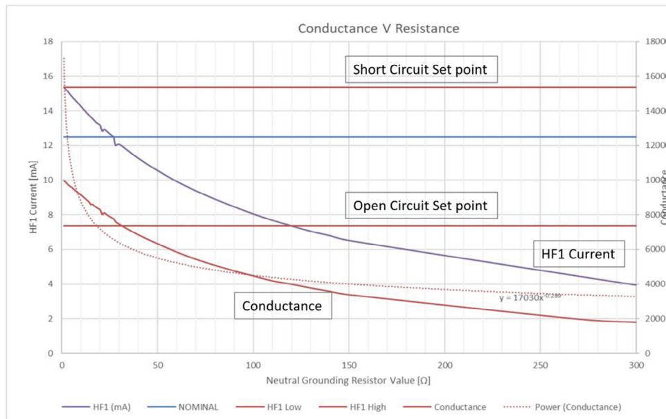
Figure 10.12: Conductance vs Resistance - HF1, Open and Short Circuit
