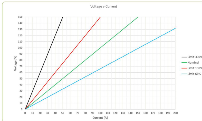
Figure 10.2: NGR Current/Voltage Graph for various Resistance Values
