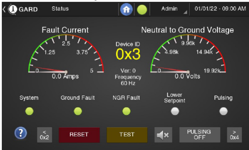
Figure 7.3: Status Screen
