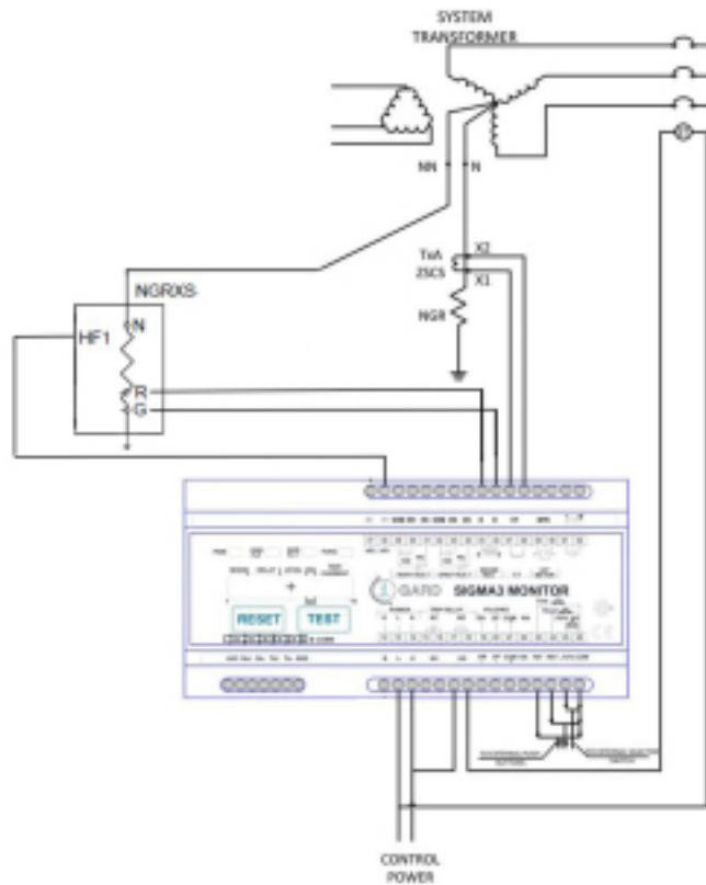
Figure 3.2: SIGMA 3 Typical System Diagram (LRG System)
