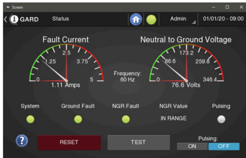
Figure 10.13: SIGMA 3 Status Screen
