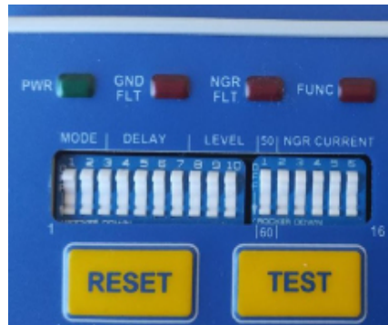
Figure 6.1: SIGMA 3 Dip Switch Array
