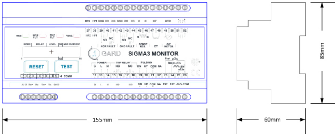
Figure 12.1: SIGMA 3 Dimensional Drawings
