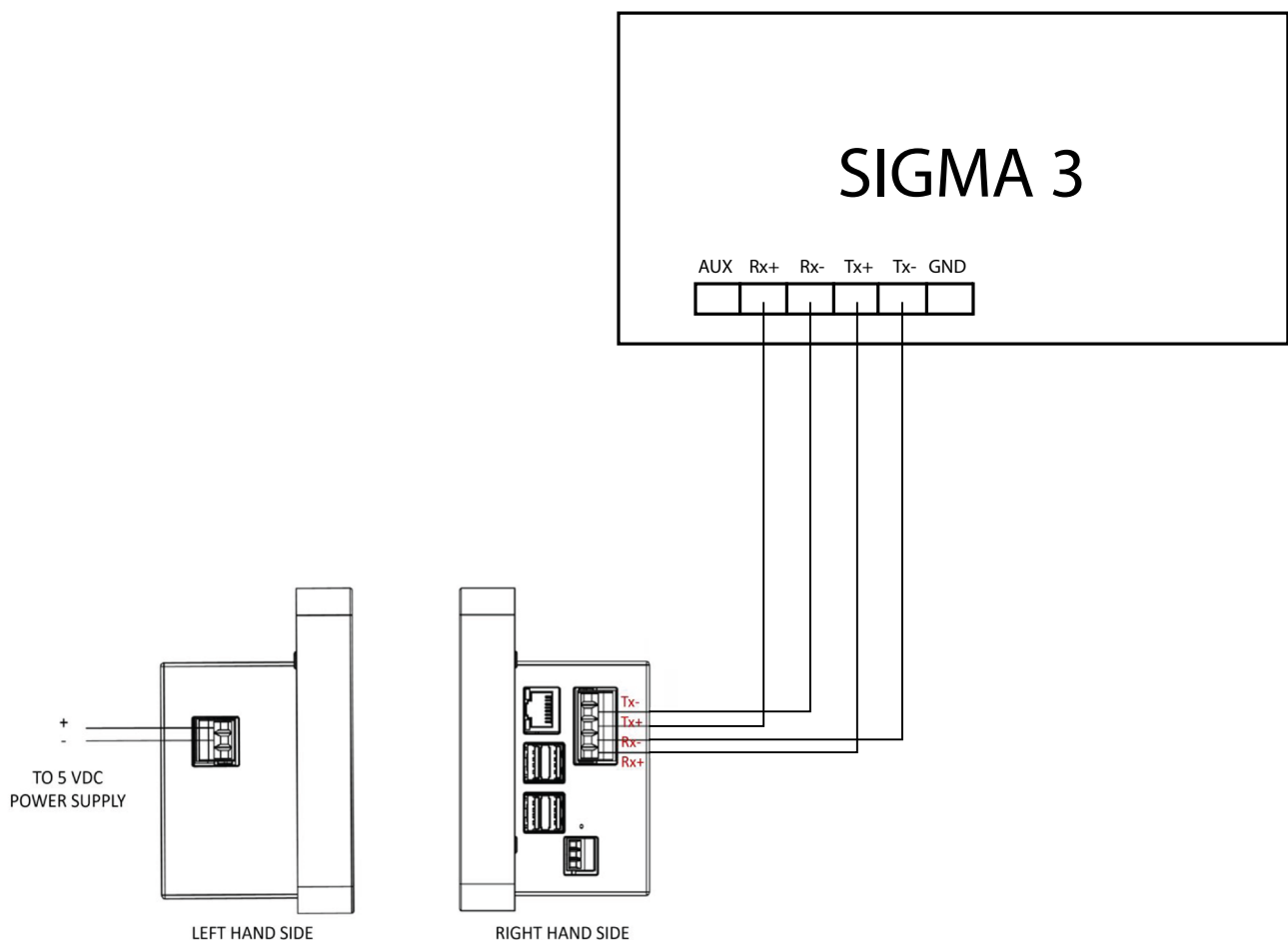
Figure 7.1: SIGMA 3 to SIGMA 3-TDM Connection Diagram
