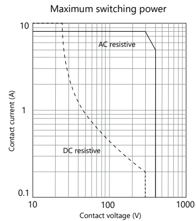
Figure 11.2: Maximum switching power Volts and Amps (AC/DC)
