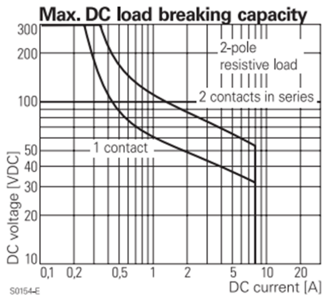
Figure 2.4.1: Maximum switching power Volts and Amps (AC/DC)
