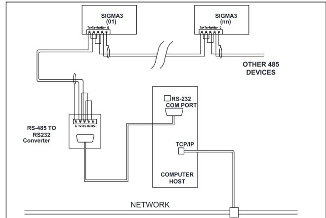
Figure 8.1 (b): Alternate 2-wire MODBUS Communication Connection
