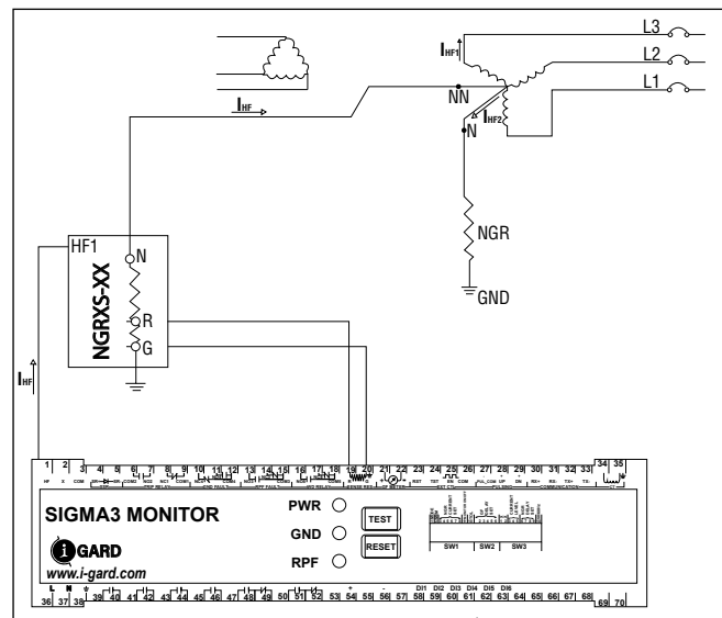
Figure 5.3.2.1: Injection Mode
